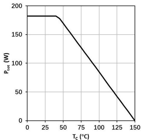
Fig. 16 Power Dissipation P_{tot} = f(T_C) , R_{\theta JC} = 0.6\text{ }^{\circ}\text{C/W}
