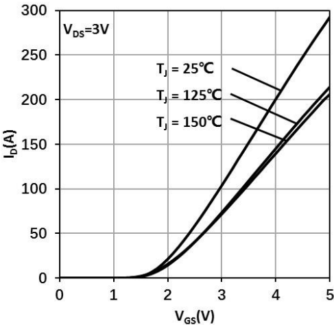
Fig. 6 Typ. Transfer Characteristics
