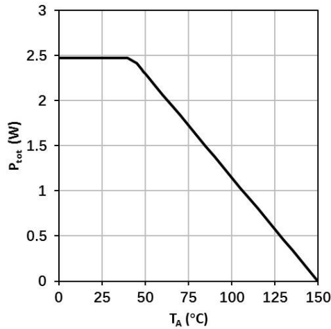
Fig. 17 Power Dissipation P_{tot} = f(T_A) , R_{\theta JA} = 43.5 \text{ } ^\circ\text{C/W}
